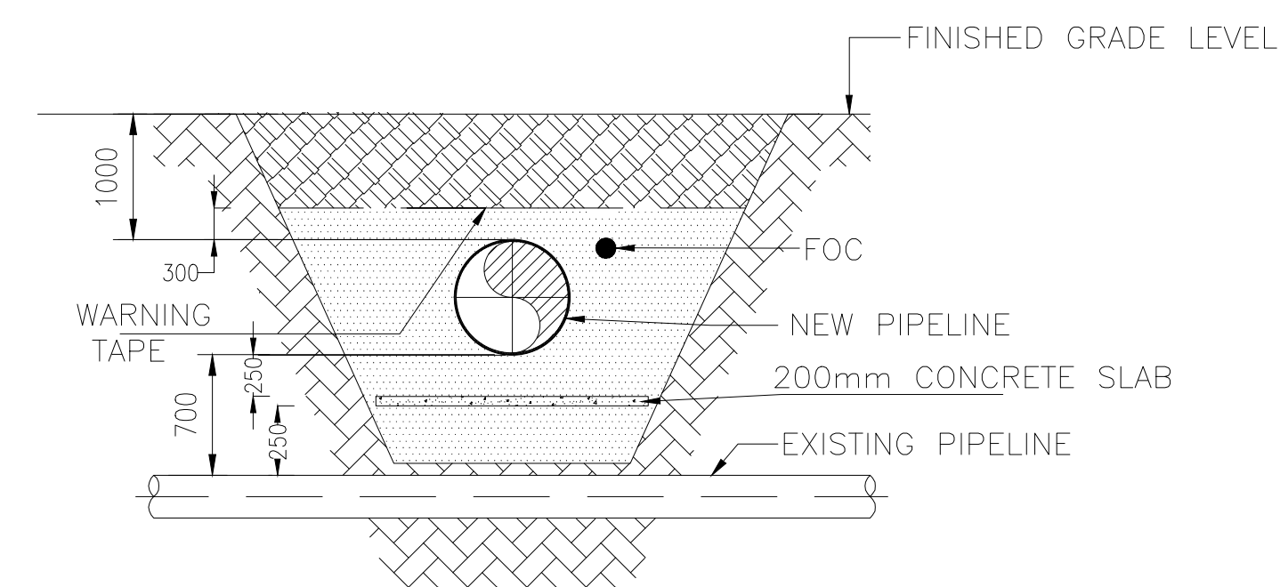
SECTION B-B
